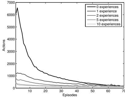
Figure 3: Learning curves for agents with agent-space options, with varying numbers of training experiences.
