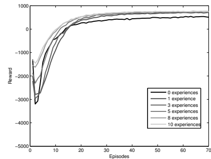
Figure 9: Learning curves for agents with both types of options, with varying numbers of training experiences.
